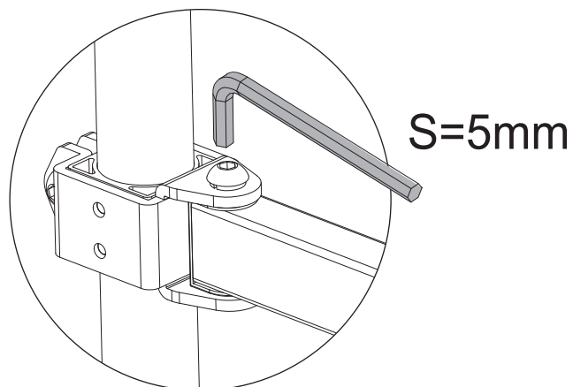
Arm Adjustment
